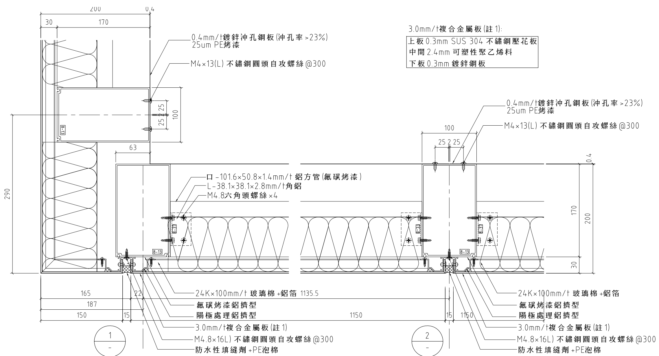
1,2 SECTION DETAIL DA-08
