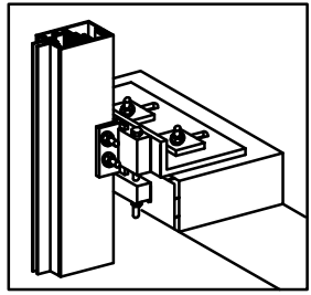
MAIN ANCHOR PART ISOMETRIC
