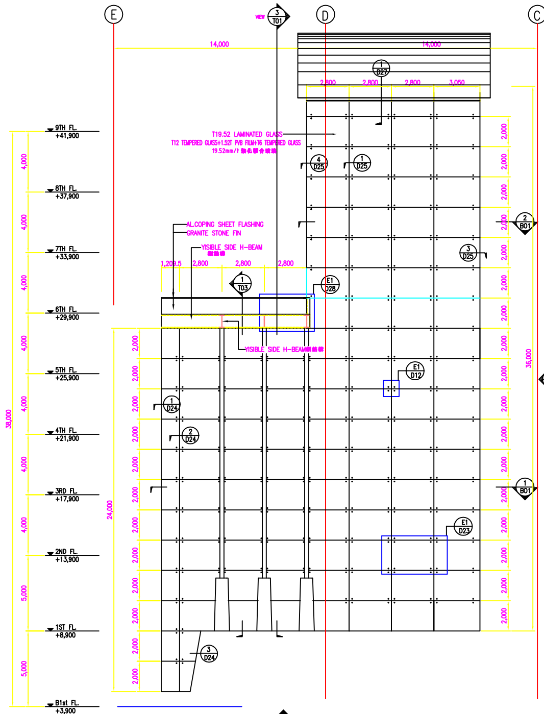
1 ELEVATION-A 幕墙立面图 T01 10~11 Line & E~C Line Scale: 1/200
